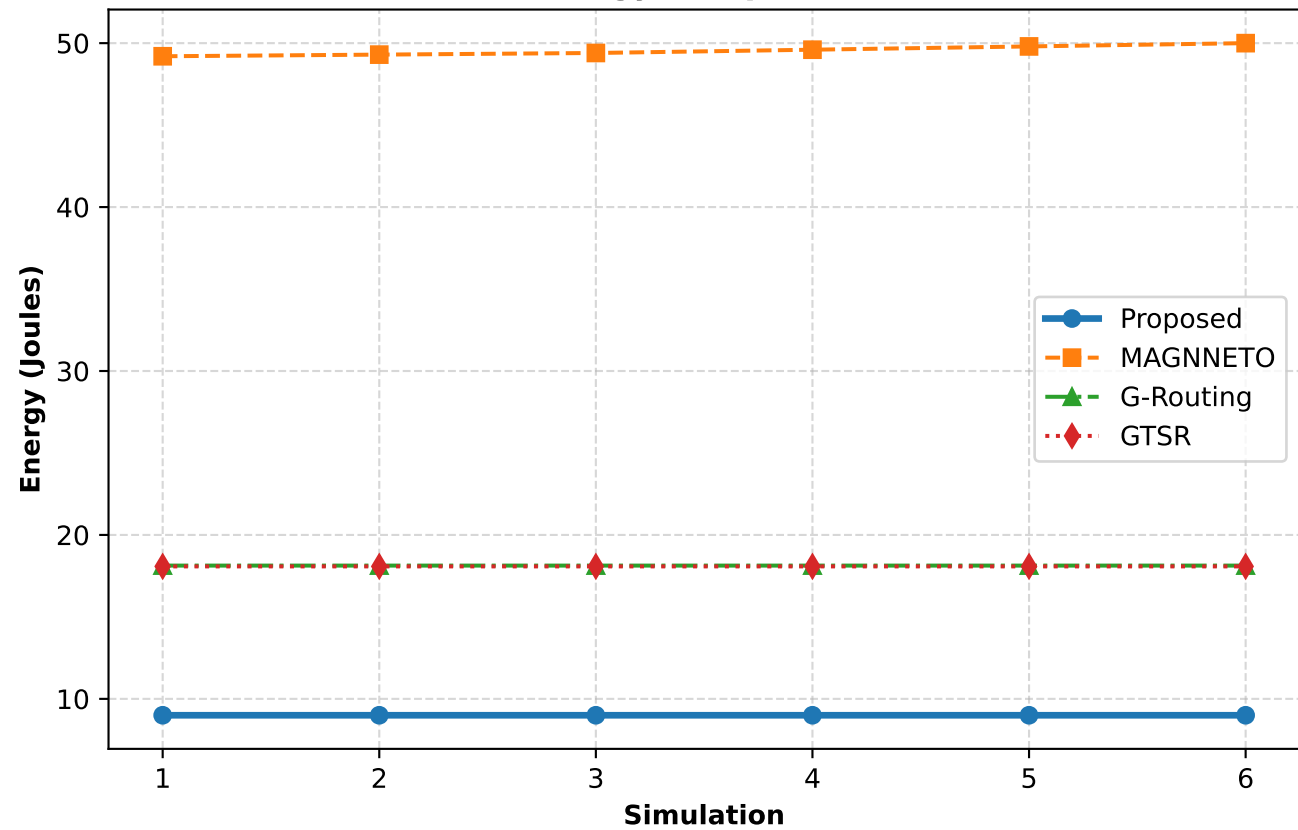
Energy Comparison
